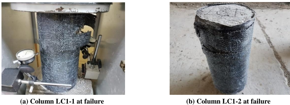
Plate 5. Modes of failure of columns LC1
