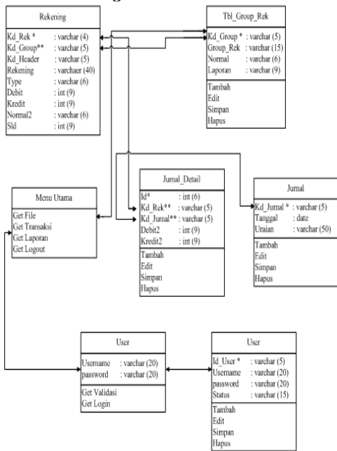
Gambar 3. Class Diagram
