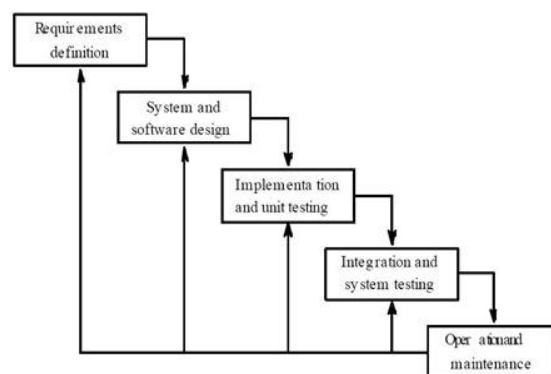
Gambar 2. Metode Waterfall
