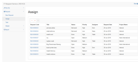
Gambar 8. Tampilan assign
