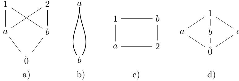
FIGURE 1. a) The poset P_1 in Example 1.1; b) The CW-complex with face poset P_1 ; c) The order complex of P_1 ; d) The poset P_2 in Example 1.2.
