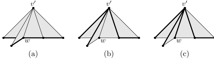
FIGURE 4. (a) A vertex with link T' = \bullet \rightarrow \bullet \rightarrow \bullet . (b) A modified embedding T'' of \bullet \rightarrow \bullet \rightarrow \bullet . (c) Extension to an embedding of T = \bullet \rightarrow \bullet \rightarrow \bullet .
