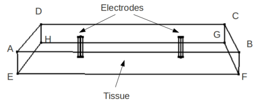
Fig. 1: Schematic of the 3D FEM model showing the tissue and electrodes, and symmetry plane defined by points ABCD
