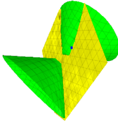
FIGURE 7.1. Transversal intersection of two implicit lightlike surfaces
