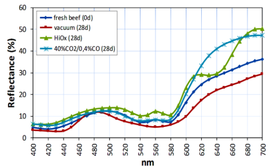
Figure 1. Reflectance spectra of fresh Longissimus dorsi beef steaks and 28 days after packaging in vacuum, HiOx-MAP and CO-MAP.
