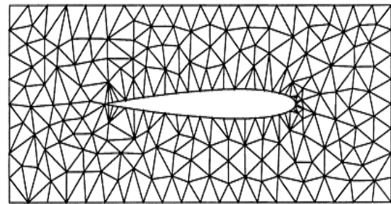
Gambar 1.3. Unstructure Mesh[8]
