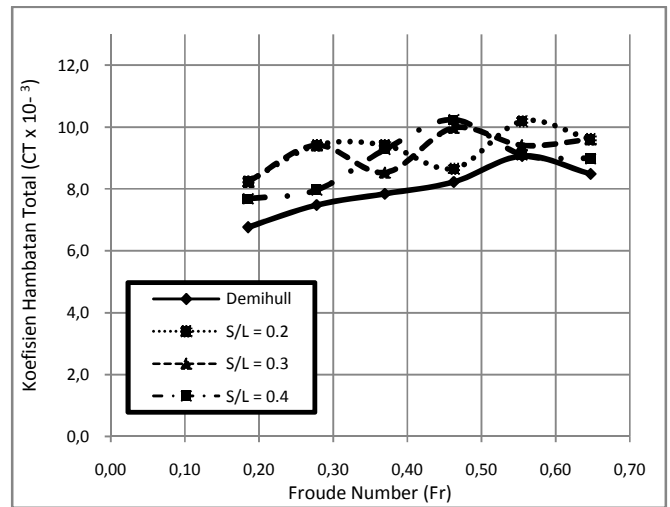
Gambar.7 Koefisien hambatan total ( Towing Tank )
