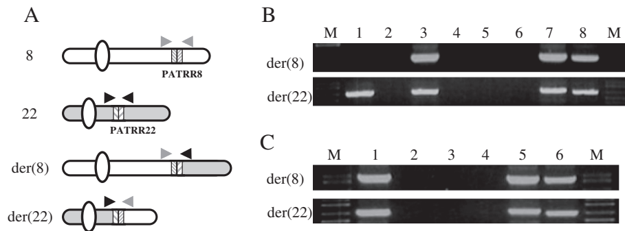
Figure 2 The der(8) and the der(22) junction fragments of the t(8;22) . A. Diagram for the translocation-specific PCR system. Chromosome 8 is indicated in white, while chromosome 22 is depicted in grey. Hatched boxes indicate PATRR arms. Translocation-specific PCR was performed with one primer designed at the flanking region of PATRR8 (grey primers) and with the other primer at the flanking region of PATRR22 (black primers). B. Results of family 1. Upper panel indicates results for the der(8) , while lower panel indicates those of the der(22) . Lane M, size markers; lane 1, FHU13-031 (proband); lane 2, FHU13-032 (father); lane 3, FHU13-033 (mother); lanes 4 and 5, normal healthy controls; lane 6, water control; lanes 7 and 8, balanced t(8;22) translocation carriers unrelated to the family. C. Results of family 2. Lane M, size markers; lane 1, FHU13-027 (proband); lanes 2 and 3, normal healthy controls; lane 4, water control; lanes 5 and 6, balanced t(8;22) translocation carriers unrelated to the family.
