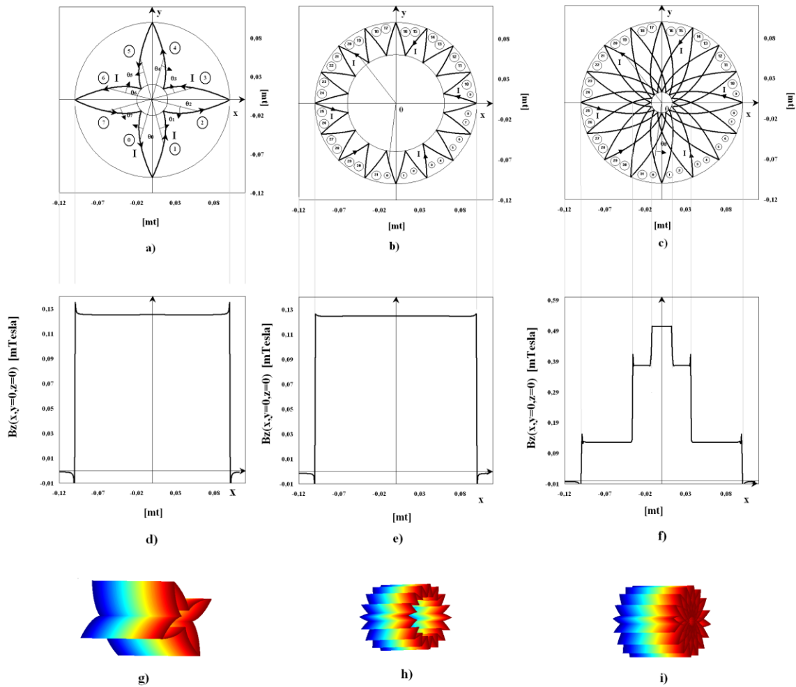
Fig. (14). a) and g) four leaf clover coil ( p=2, M=1, q=0 ) b) and h) crown solenoid ( p=4, M=1, q=0 ) c) and i) crown ( p=4, M=4, q=0 ), d) and e) , f) B_z versus x at y = 0, z = 0 four leaf clover, crown solenoids, g) and h) , i) figures were obtained by using MATLAB).
