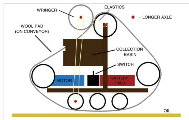
Figure 1. Oil skimmer, side profile
