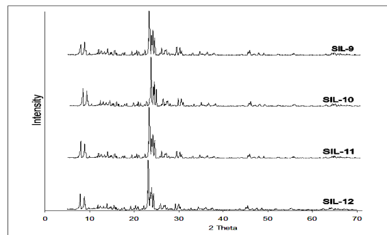
Figure 5. XRD patterns of silicate-1 crystals
