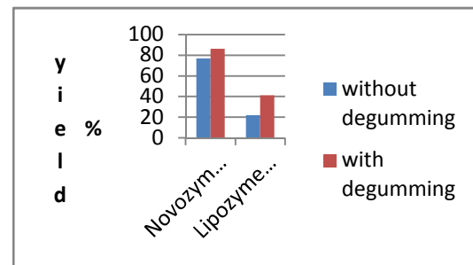
Figure 2. Lipase screening for CPO transesterification
