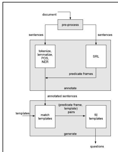
Gambar. 2. Kerangka kerja question generation Lindberg dkk[3]
