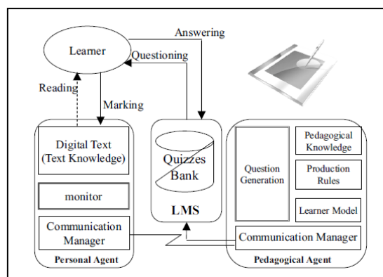
Gambar 1. Kerangka question generation Iwane dkk [2]
