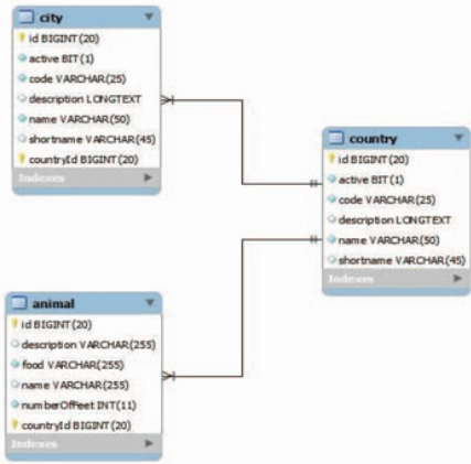
Figure 4 ERD for HCE Usage
