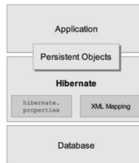
Figure 2 Hibernate Architecture [11]
