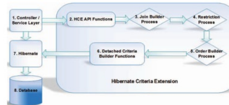
Figure 3 HCE Architecture
