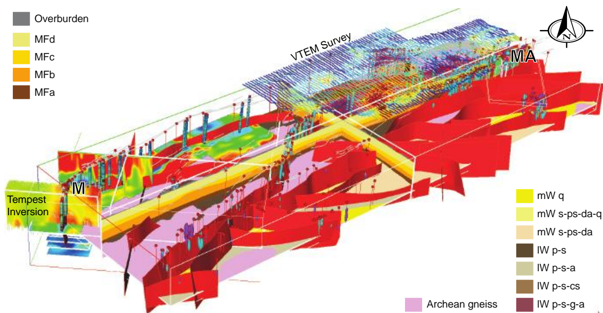
Figure 12: Parts of the CEM for the McArthur River – Millennium area showing basement and basin geology, faults (subvertical red planes), locations of diamond drill cores (lithology, whole-rock geochemistry, hyperspectral mineralogy, and petrophysics), a VTEM® survey over the NE part, and a Tempest® inversion around Millennium. M: Millennium, MA: McArthur River; MFa, MFb, MFc, MFd: members of the Manitou Falls Formation, uW, mW, IW: upper, middle, and lower parts of the Wollaston Group, a: arkose, da: dirty arkose, cs: calc-silicate, g: graphitic sections, p: pelite, ps: psammite, q: quartzite, s: semipelite.
