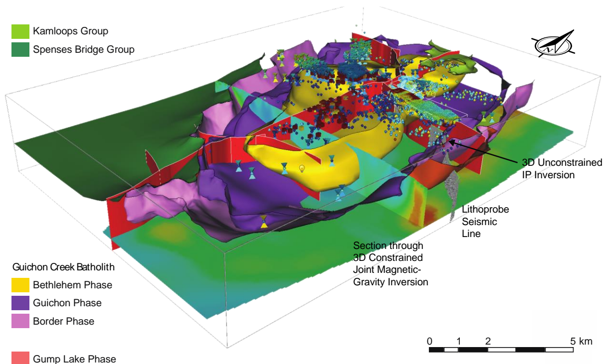
Figure 15: Parts of the CEM for the Highland Valley area showing geology, faults (subvertical red), geochemical samples (small diamonds), SWIR mineralogical samples (small cubes), petrophysical measurements (large hourglasses), a 3D unconstrained IP inversion, a slice through a 3D constrained joint magnetic-gravity inversion, and the location of a Lithoprobe seismic line. Bethsaida, Chataway, and Skeena phases of the batholith are not shown for clarity.
