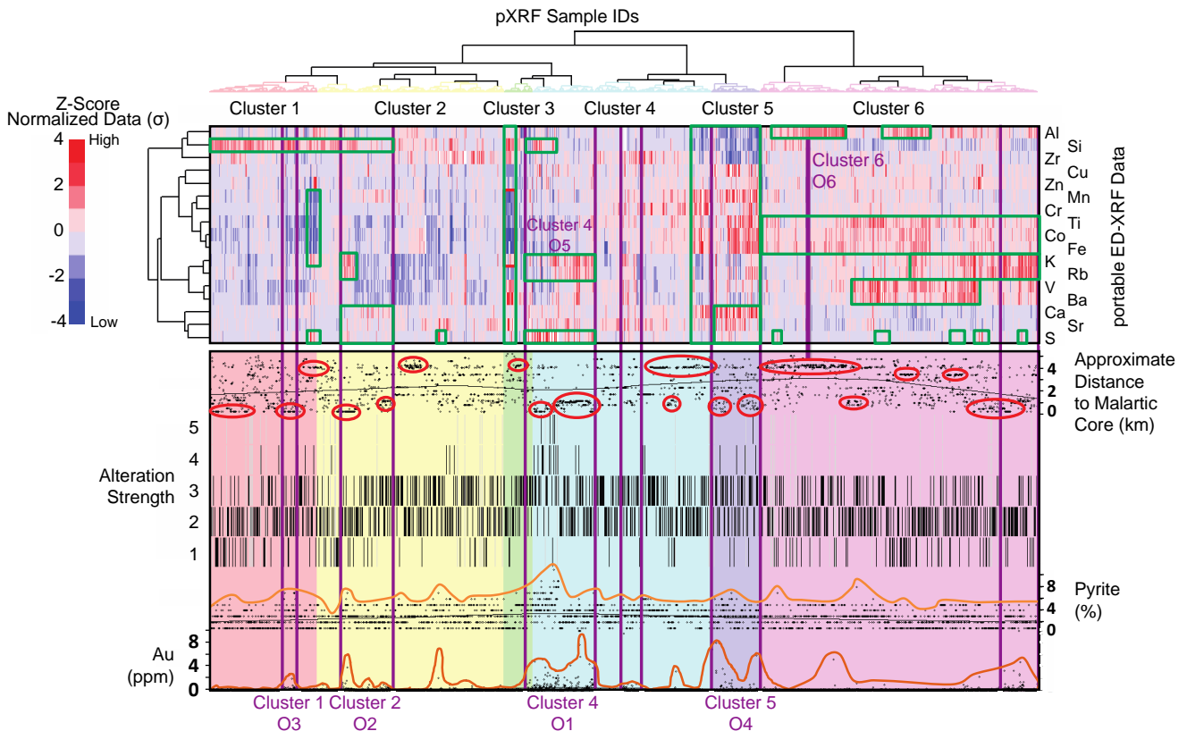
Figure 3: Clustered Heat Map (CHM) visualization for 3787 samples of Pontiac Group metasediments from the Canadian Malartic Mine area (modified after Feltrin et al., 2016). The upper section shows CHM of normalized portable-XRF data with colour-scale indicating relative element abundance (warmer colors for higher abundances), broken down into six broad clusters. The lower section shows 1) estimated Euclidean distance from the approximate centre of high-grade Au-mineralization, 2) logged alteration strength (1 lowest, 5 highest), 3) logged pyrite abundance, and 4) analyzed Au abundance (fire assay). Purple squares outline additional mineralized subclusters, representing internal heterogeneities in the broad clusters. O1–O6 highlight specific observations within those subclusters. Red circles outline subpopulations of samples occurring at the same/similar distance from the deposit hypothetical centre. Green squares outline key subclusters (squared rows capture high-abundance groups, squared columns capture particularly distinctive specimen groups). By comparing clusters/subclusters against Au abundance and other alteration indicators it is possible to interpret if a cluster is likely linked to mineralization/alteration. For example, in some cases high Si appears to have a positive relationship with mineralization/alteration (e.g., Cluster 4 – O1), but some samples with elevated Au may have low Si if other alteration phases are dominant (e.g., Cluster 4 – O1 has more K-altered samples, Cluster 2 – O2 has more abundant Ca-altered samples). High Fe is often associated with high S (confirmed by peaks in pyrite abundance), but sometimes also with high Ca-Sr-Mn, likely indicating the presence of Fe-bearing carbonates. High K-Rb correlate well with mineralization/alteration in most cases, except in zones dominated by high Si (Cluster 1 – O3) or carbonate alteration (Cluster 5 – O4). High K-Rb samples occur predominantly in proximal locations (e.g., Cluster 4 – O5), suggesting that K-altered rocks are more likely to represent near-core assemblages. A CHM also allows the detection of enrichments in the relative abundance of elements distal to and unrelated to mineralization (e.g., Cluster 6 – O6 for Al).
