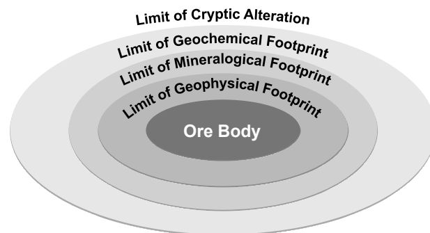
Figure 1: Schematic representation of a multi-parameter ore system footprint, each of which may be internally zoned and extend to different distances with a geometry that may vary according to structural controls on magmatic/hydrothermal fluids or deformation, metamorphism, erosion, and glacial cover.
