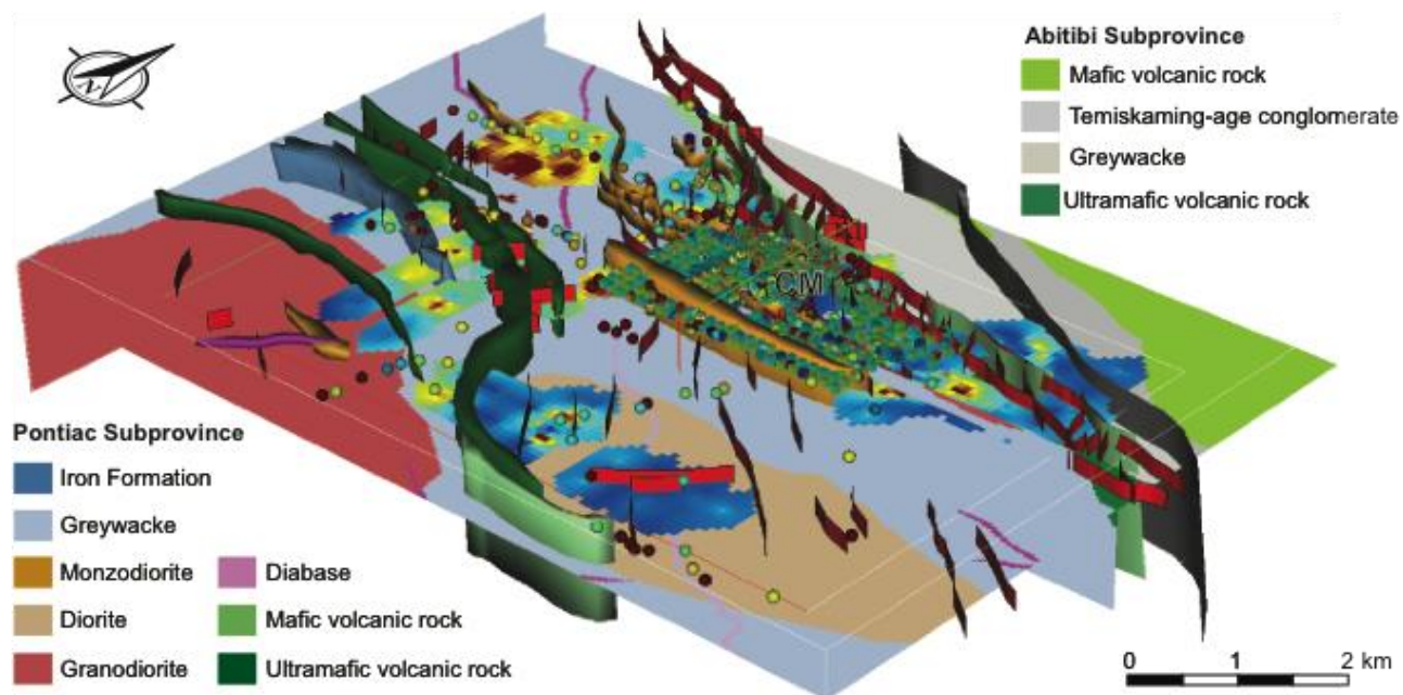
Figure 9: Parts of the CEM for the Canadian Malartic area showing geology, locations of faults (irregular subvertical red-rust-black planes), geochemical-mineralogical-petrophysical samples (small coloured spheres), pXRF lithochemistry-hyperspectral mineralogy samples (small coloured cubes in mine area), and IP surveys (blue-yellow-brown coloured horizontal grids).
