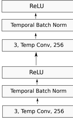
Figure 2: Convolutional block.
