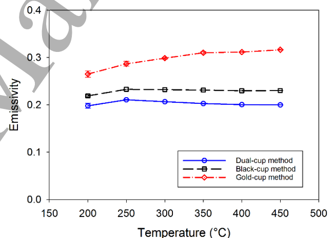
Figure 14. Emissivity of polished SS304.
