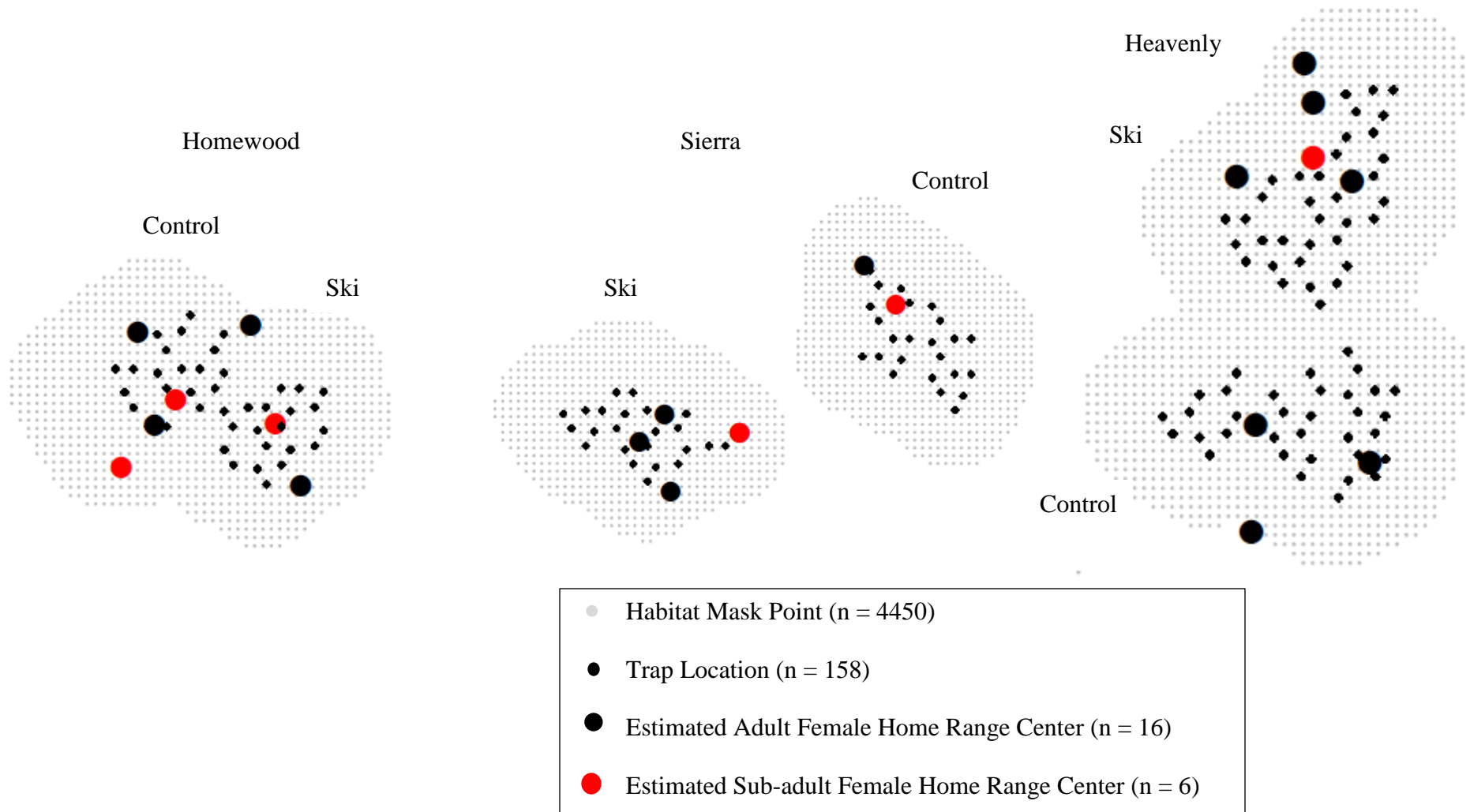
Figure 3-2. Estimated home range centers from a spatially explicit capture-recapture analysis using SECR for female Pacific Martens ( Martes caurina ) on 3 pairs of ski and control study areas in the Lake Tahoe region of California and Nevada.
