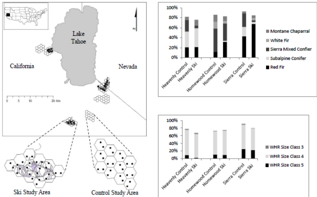
Figure 2-1. Location of the paired ski and control Pacific marten study areas and their sampling locations (dots) and ski runs (gray lines) in the Lake Tahoe Region of California and Nevada, USA (A). Habitat compositions of each paired ski and control study area (B) using the California Wildlife Habitat Relationships (WHR) classification and remotely sensed data available from the United States Forest Service Pacific Southwest Region Remote Sensing Lab's existing vegetation coverage (updated 2010). The WHR size classes (C) refer to the following tree diameter at breast height classes: 3 (15–28 cm), 4 (28–61 cm), and 5 (>61 cm).
