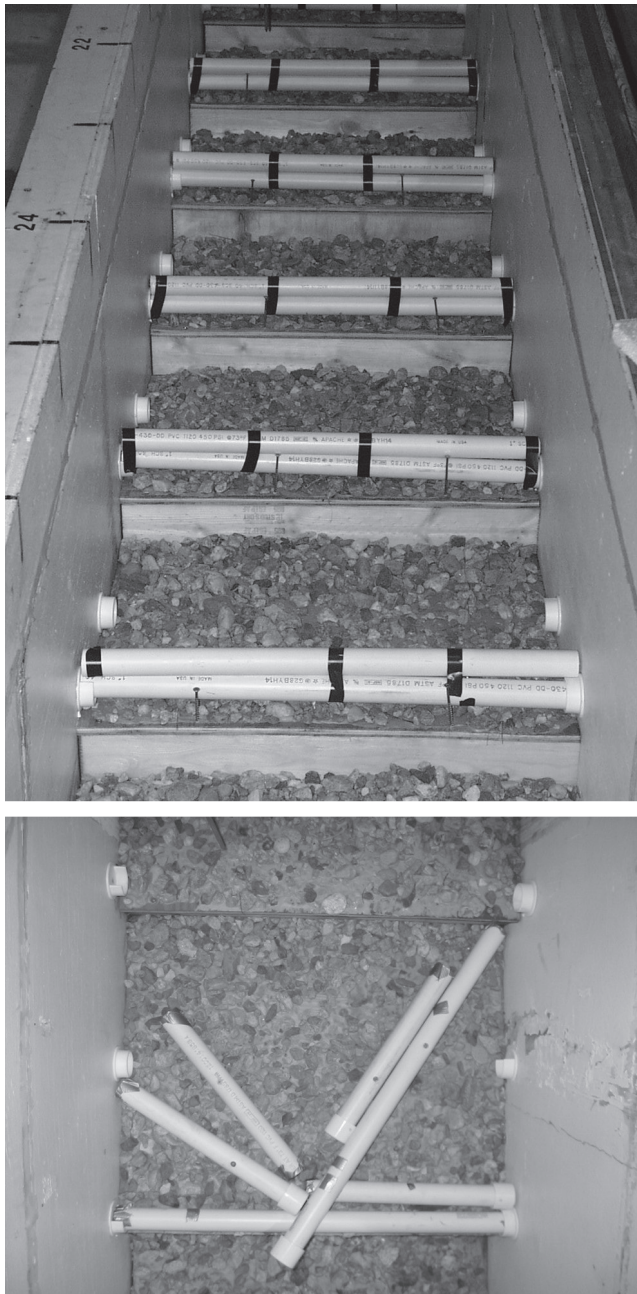
Figure 4. Two LWD arrangements assessed as part of factorial tests of the effect of LWD configuration on flow resistance: (top) stacked (high density, perpendicular) and (bottom) jams. Single pieces were also tested, as shown in Figures 2 and 3.
