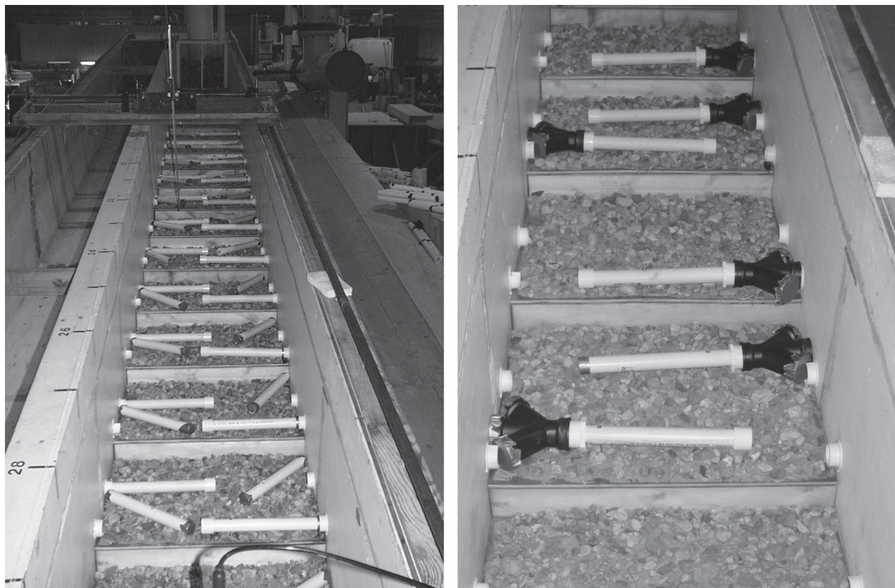
Figure 3. Upstream view of flume, showing examples of LWD configurations employed to test effects of piece length on flow resistance: (left) short pieces (high density, combination orientation) and (right) rootwad pieces (high density, perpendicular orientation). Long pieces were also tested, as shown in Figure 2.
