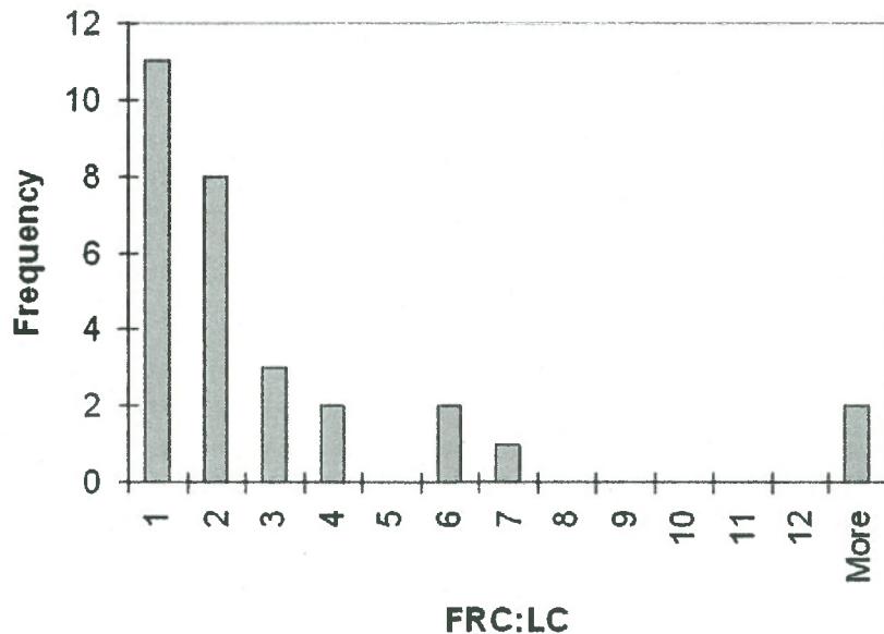
Figure A1. Frequency histogram of the ratio of new fine root carbon to new leaf carbon.
