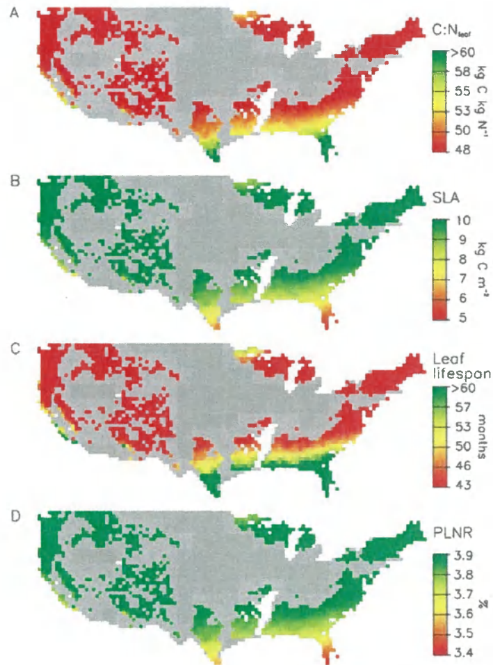
Figure 3. ENF parameter variation in the continental United States: (a) C:N_{\text{leaf}} ( \text{kg C kg N}^{-1} ), (b) specific leaf area (SLA, \text{kg C m}^{-2} ), (c) leaf life span (months), and (d) the percent of leaf nitrogen in Rubisco (PLNR, dimensionless). Gray areas do not contain ENF in the VEMAP dataset.
