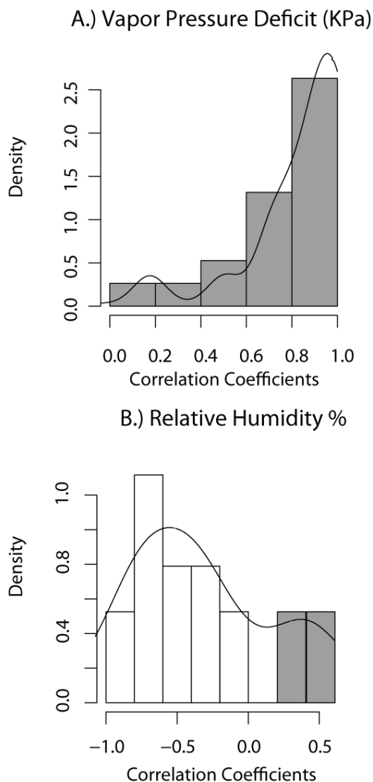
Fig. 4. Density functions of Pearson correlation coefficients. Correlation coefficients are reported for relationships between \delta_s and vapor pressure deficit ( A. ) as well as relative humidity ( B. ). Probability density functions (black lines) are superimposed on histograms (boxes) where positive relationships are indicated by positive correlation coefficients (grey bars) and negative relationships are indicated by negative correlation coefficients (white bars). See Table 1 for actual correlation coefficients.
