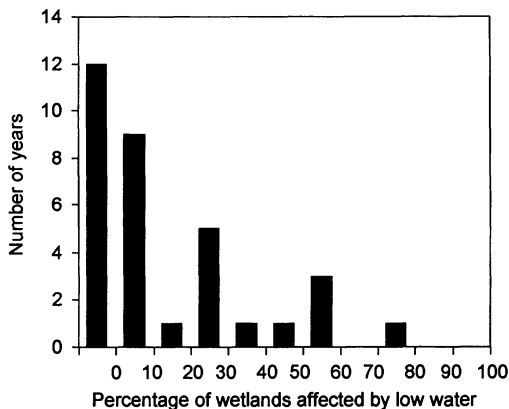
FIGURE 1. The extent to which low water events were widespread among 13 south Florida wetlands used by Snail Kites over a 33-year period (1965–1997), as indicated by the number of years in which wetlands experienced concurrent low water events.
