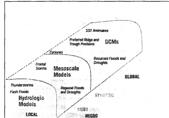
Space-time scales of interest in hydrology (Hirshboeck 1988).
