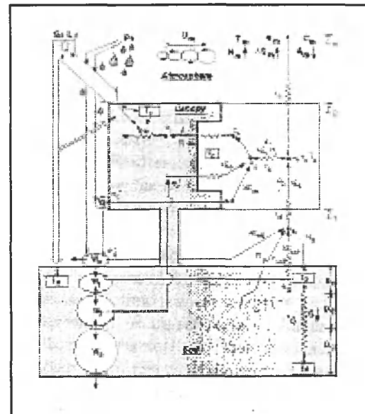
Schematic diagram depicting most of the processes modeled in SIB 2.
