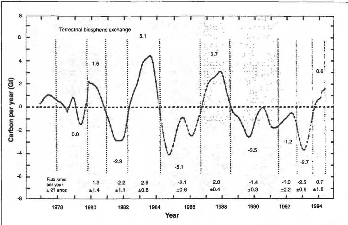
Interannual variability in terrestrial biospheric net CO 2 exchange, computed from the network of flask sampling of atmospheric CO 2 and an atmospheric transport model (Keeling et al. 1995).
