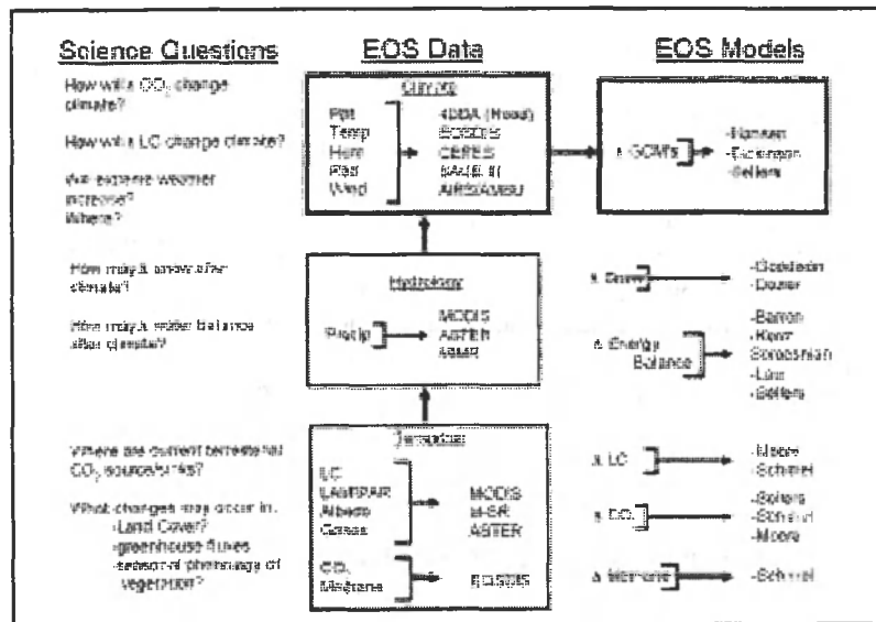
A summary diagram of land-climate research in EOS.
