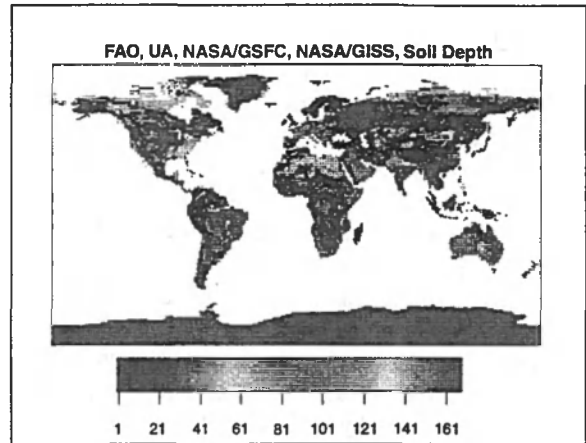
A global database of soil depth. This 1^\circ \times 1^\circ data set, developed by the ISLSCP Initiative 1 project, is used in global climate, hydrologic, and biogeochemical modeling (Sellers et al. 1996).
