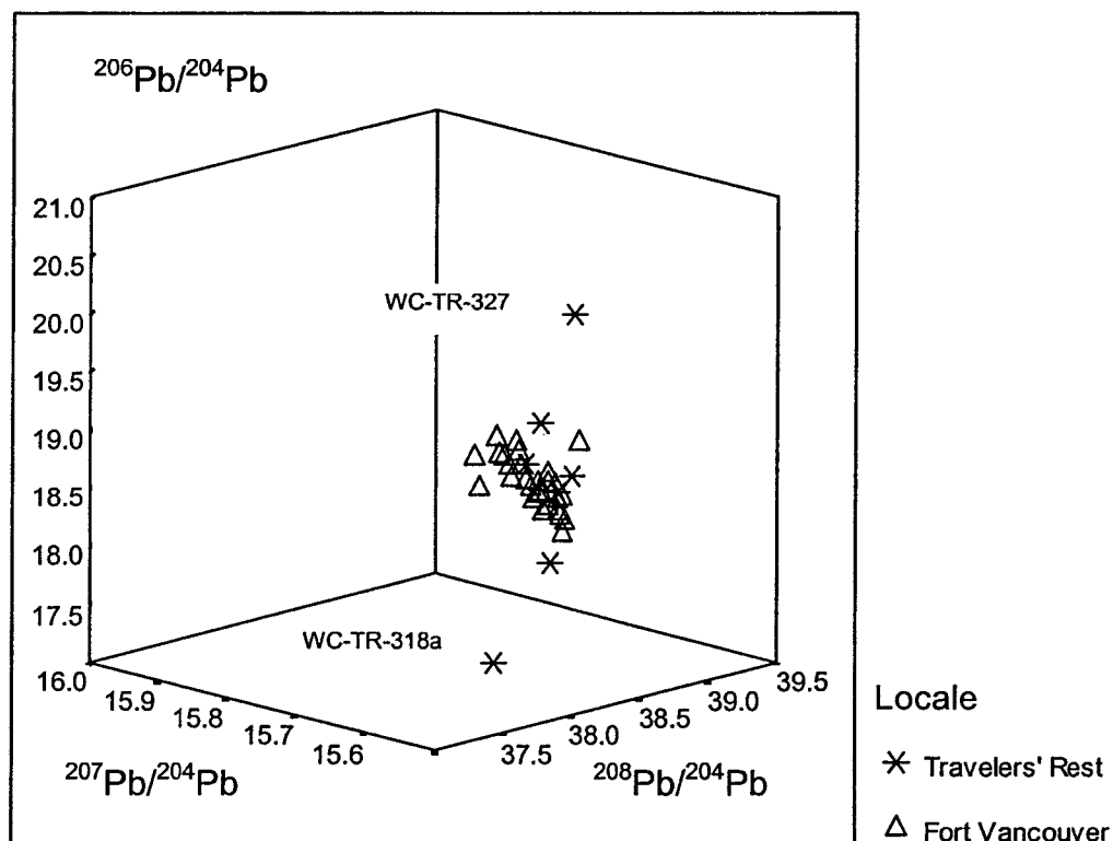
Figure 4-3 Trivariate plot of the lead Fort Vancouver and Travelers' Rest artifacts (n = 36). The lead isotope ratios serve as the three axes: x-axis is ^{207}\text{Pb}/^{204}\text{Pb} , y-axis is ^{206}\text{Pb}/^{204}\text{Pb} , and z-axis is ^{208}\text{Pb}/^{204}\text{Pb} .
