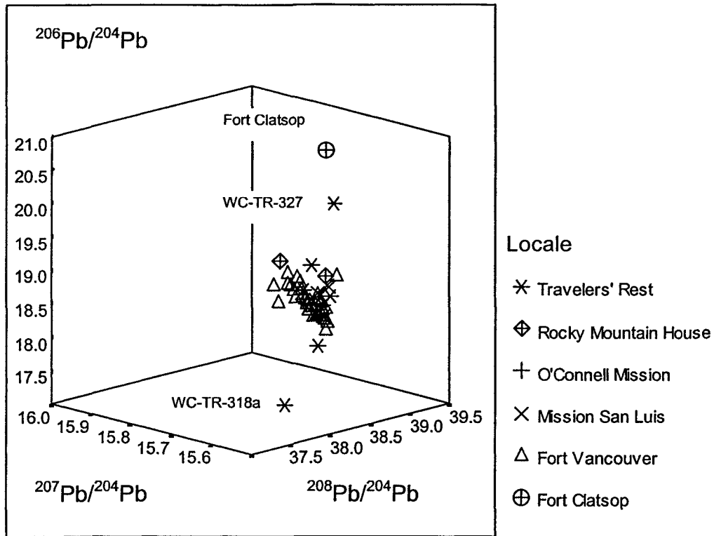
Figure 4-2 Trivariate plot of lead artifacts only (non-lead artifacts and modern bullets excluded) (n = 56). The lead isotope ratios serve as the three axes: x-axis is ^{207}\text{Pb}/^{204}\text{Pb} , y-axis is ^{206}\text{Pb}/^{204}\text{Pb} , and z-axis is ^{208}\text{Pb}/^{204}\text{Pb} .
