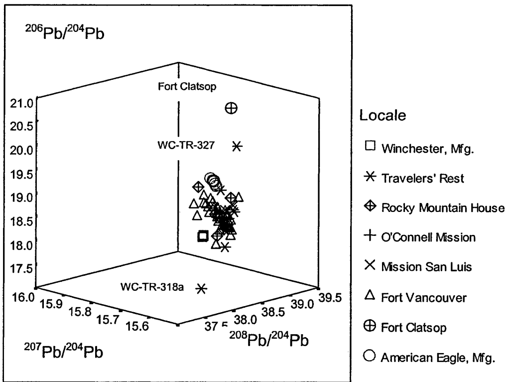
Figure 4-1 Trivariate plot of all artifacts (n = 76) under consideration (numbered data points discussed in text). The lead isotope ratios serve as the three axes: x-axis is ^{207}\text{Pb}/^{204}\text{Pb} , y-axis is ^{206}\text{Pb}/^{204}\text{Pb} , and z-axis is ^{208}\text{Pb}/^{204}\text{Pb} .
