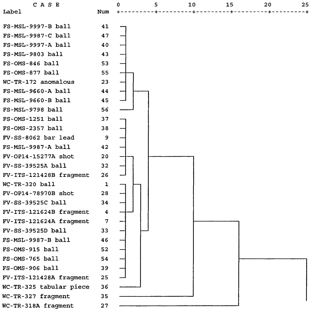
Figure 4-5 Portion of cluster analysis based on lead isotope data for all known lead artifacts (see Appendix D for complete diagram) (n = 56).
