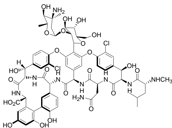
23 , Vancomycin
