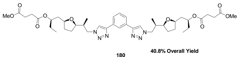
Figure 6.8: Synthesis of 1,3-bis-triazole-bis-ester homononactic acid analogue 180 .
