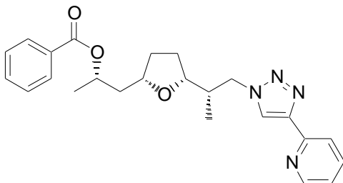
81, Minus 1,4-Regioisomer
