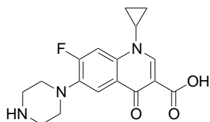
28 , Ciprofloxacin
