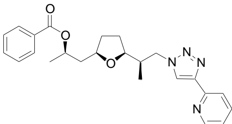
72, Racemic 1,4-Regioisomer
