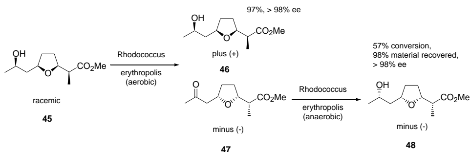
Scheme 2.2: The Rhodococcus erythropolis enzymatic separation of methyl ( \pm )-nonactate 45 into 46 and 48 . [7]
