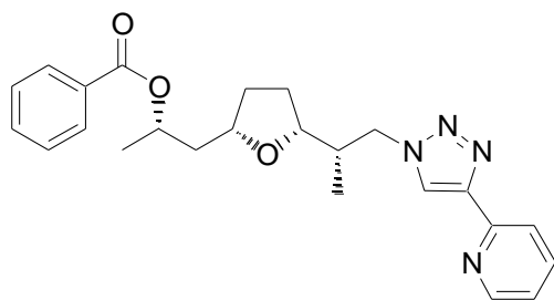
81, Minus 1,4-Regioisomer
