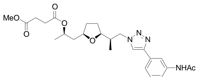
71, Racemic 1,4-Regioisomer
