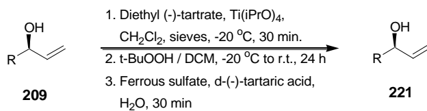
Scheme 8.3: General synthesis of (S)-phenyl substituted vinyl secondary alcohols 221 .
