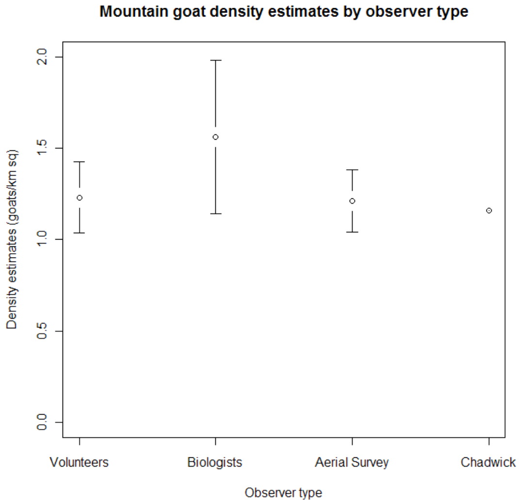
Fig. 6: Density estimates of mountain goats by volunteers, biologists, aerials surveys and previous research (Chadwick 1977) in Glacier National Park, Montana derived from N-mixture models with confidence intervals where available. Confidence intervals for aerial survey estimates are derived using a range of detection probabilities (0.55- 0.91) from other mountain goat aerial surveys (Gonzalez-Voyer et al. 2001; Rice et al. 2009) as a hypothetical correction factor for our aerial survey count.
