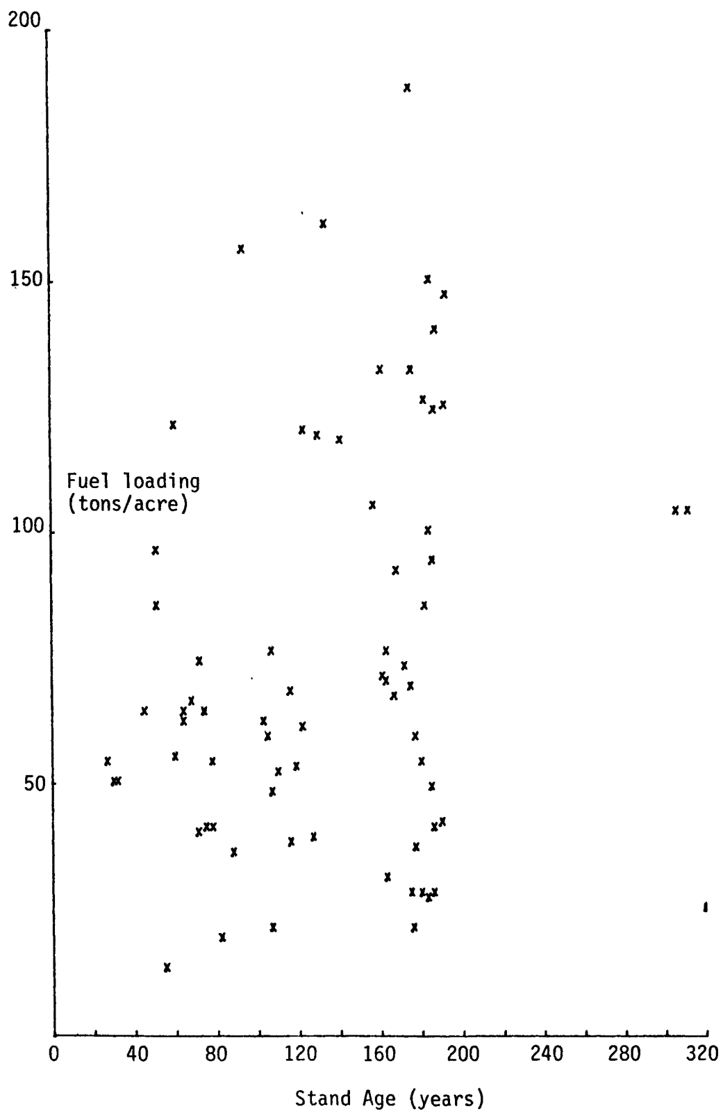
Figure 1 = Fuel loading vs. stand age for 71 Lodgepole Pine stands. East Fork Bitterroot drainage, Montana
