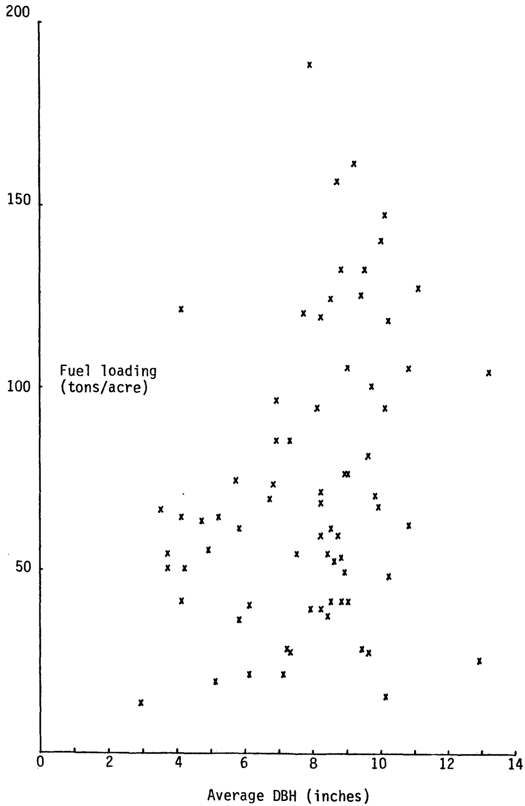
Figure 2 = Fuel loading vs. average DBH for 71 Lodgepole Pine stands. East Fork Bitterroot River drainage, Montana
