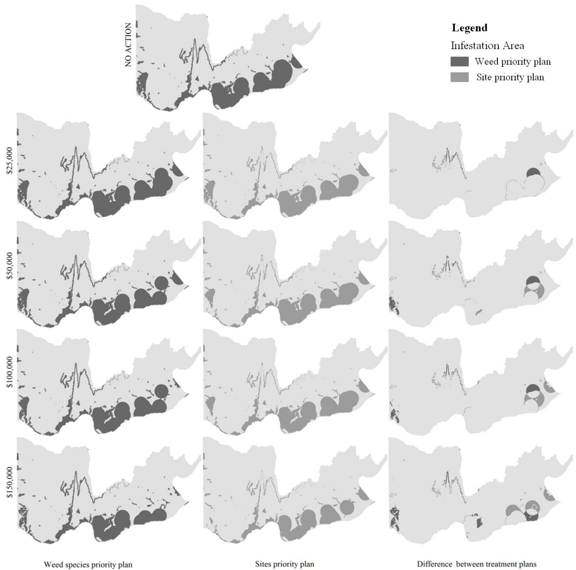
Figure 1.10. Predicted infestation areas at the end of five-year planning horizon resulting from each of the treatment plan alternatives.
