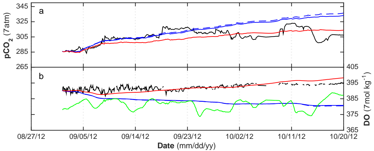
Figure 4.1. ITP-64 p\text{CO}_2 and DO data (black) and model time-series data calculated from modeled gas exchange using the ice cover (blue solid) shown in Fig. 3.1 and without ice cover (blue dashed). Modeled gas exchange plus NCP assuming the residual signal is all NCP are shown (red). The green line corresponds to the equilibrium concentration of \text{O}_2 at in situ temperature, salinity and atmospheric pressure.
