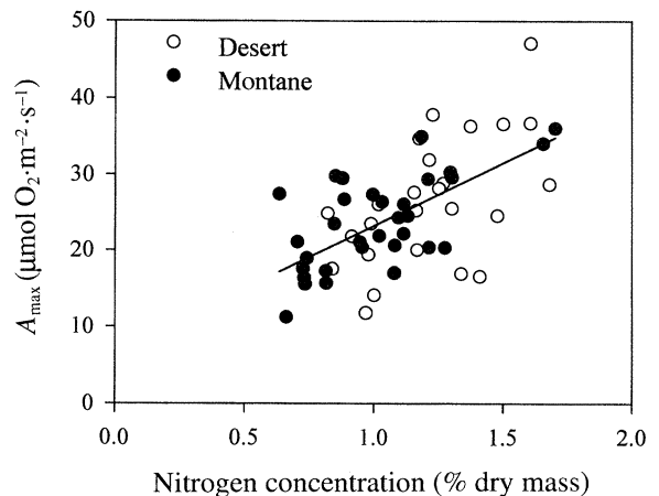
FIG. 5. Photosynthetic capacity ( A_{\text{max}} ), measured as \text{O}_2 evolution, as a function of leaf nitrogen concentration in montane ( n = 32 needle samples) and desert ( n = 27 needle samples) ponderosa pine populations. For environments combined, A_{\text{max}} = 2.16 + 19.98(\%N) , R^2 = 0.47 , P < 0.001.
