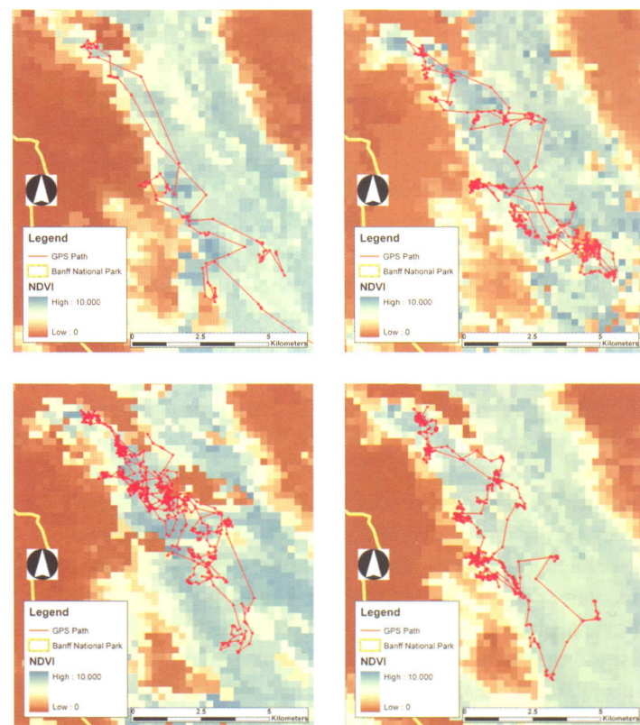
Figure 2. A Global Positioning System tracks movements of a collared female elk following mountain snowmelt patterns in the Canadian Rocky Mountains. Data show movements following green-up of forage as indexed by the Normalized Difference Vegetation Index (NDVI) from the MODIS satellite in 16-day periods in 2004 from (clockwise from top left) 24 May to 8 June, 9 to 25 June, 26 June to 11 July, and 12 to 27 July 2004.
