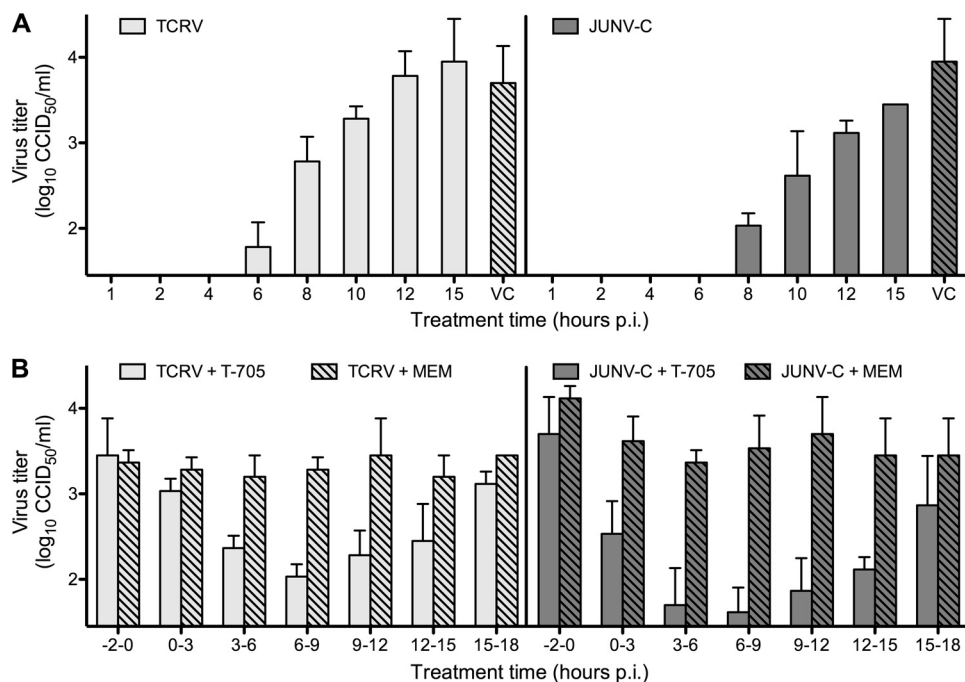
FIG. 2. Time of addition of T-705 to arenavirus-infected Vero cells. (A) For method 1, Vero cells were infected with TCRV or JUNV-C and at indicated times ( x axis) T-705 was added to infected cells at a final concentration of 200 \mu M. Infected cells exposed to MEM lacking T-705 (virus control [VC]) were included for comparison. Supernatants were collected 24 h p.i., and virus yields were determined. (B) For method 2, Vero cells were infected with TCRV or JUNV-C, and at indicated time intervals ( x axis) T-705 or MEM vehicle was added to infected cells at a final concentration of 400 \mu M. Supernatants were collected and virus yields determined as described above. Data shown are representative of three or four independent experiments per method for each virus, and error bars represent standard deviations for triplicate samples.
