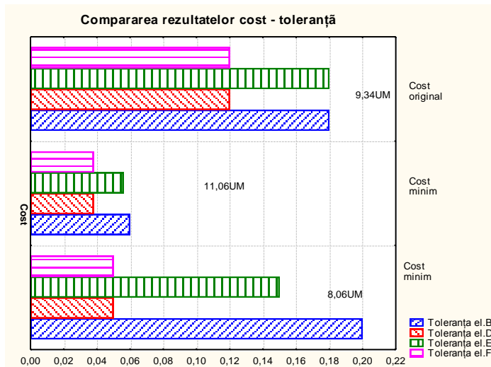
Fig. 2. Comparison of the results between tolerance and cost
