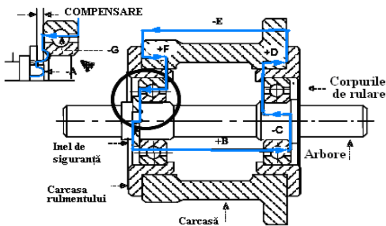
Fig. 1. Bearings assembly on an axle.
