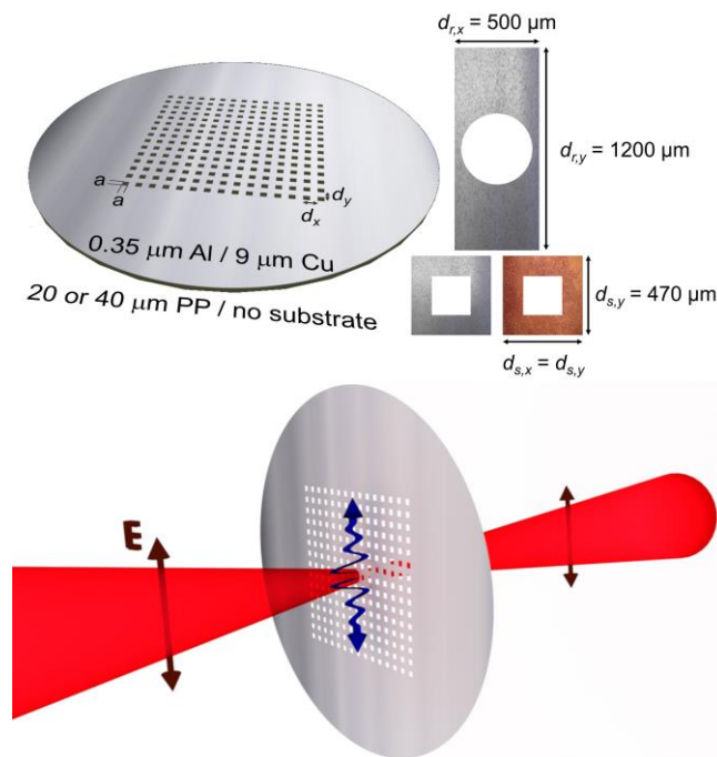
Figure 1. (top left) Schematic diagram of the subwavelength hole array in a square lattice. The metal thickness is 0.35\ \mu\text{m} and 9\ \mu\text{m} for the Al and Cu samples, respectively. The Al sample is patterned on a 20\ \mu\text{m} or 40\ \mu\text{m} thick PP film, whereas the Cu sample is freestanding. The overall diameter of the sample is 50\ \text{mm} in all cases. The sample lies in the xy plane with the linearly-polarized THz beam incident in the z -direction either focused or collimated. (top right) Unit cells of the circular hole array in a rectangular lattice with hole diameter a_r = 420\ \mu\text{m} and lattice constants d_{r,x} = 500\ \mu\text{m} , d_{r,y} = 1200\ \mu\text{m} –top– and the square hole array in a square lattice with d_{s,x} = d_{s,y} = 470\ \mu\text{m} and aperture side a_s = 230\ \mu\text{m} –bottom–. (bottom) Schematic diagram of the experimental setups.
