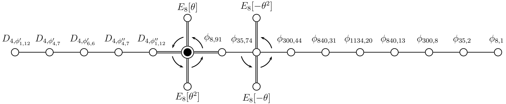
FIGURE 14. Brauer tree of the \Phi_{18} -block of E_8(q) associated to ({}^2A_2(q), \phi_{21})
