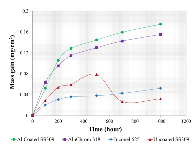
Figure 2. Discontinuous mass measurements for aluminised SS309, AluChrom 318, Inconel 625, and uncoated SS309 in 3 vol% H 2 O humidified air at 850 °C.
