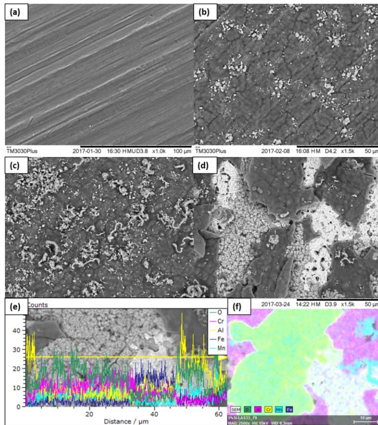
Figure 6. SEM images of aluminized SS309 exposed at 850 °C for: (a) 0 hour, (b) 100 hours, (c) 500 hours, and (d) 1000 hours. EDX line scan (e) and EDX maps (f) from the steel through the oxide scale of the aluminized SS309 after 1000 hours of exposure at 850 °C.
