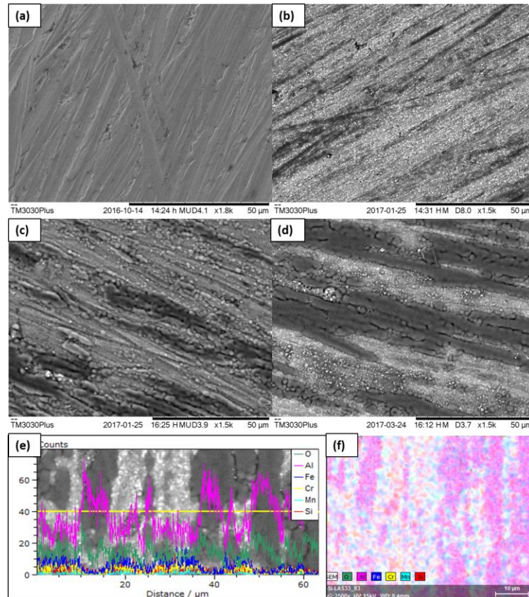
Figure 8. SEM images of AluChrom 318 exposed at 850 °C for: (a) 0 hour, (b) 100 hours, (c) 500 hours, and (d) 1000 hours. EDX line scan (e) and EDX maps (f) from the steel through the oxide scale of the AluChrom 318 after 1000 hours of exposure at 850 °C.
