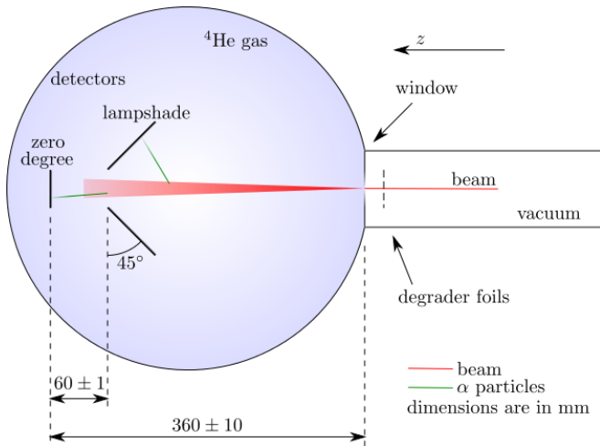
FIG. 1. (Color online) Schematic of the experimental chamber.
