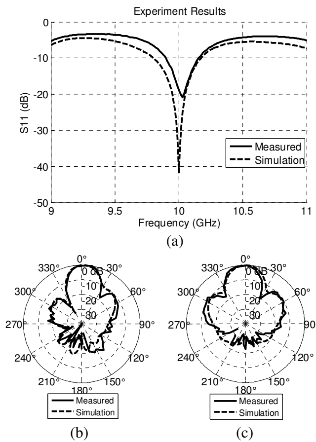
Fig. 5. Simulation and measured results of the antenna shown in Fig. 2(c); (a) return loss and far-field pattern at 10GHz in (b) E-plane and (c) H-plane
