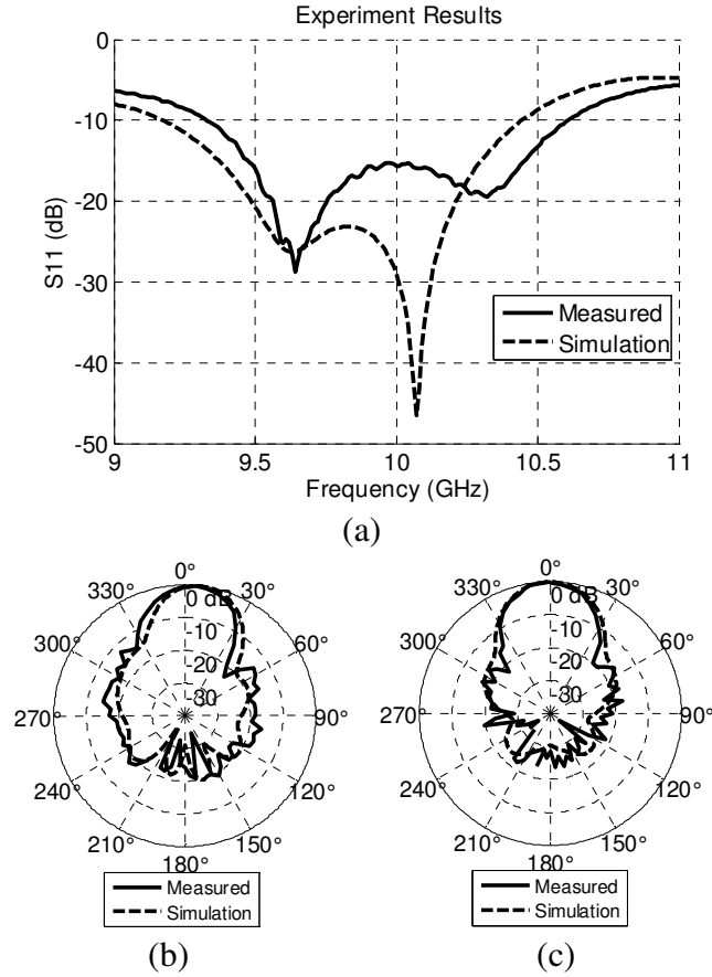
Fig. 6. Simulation and measured results of the antenna shown in Fig. 2(d); (a) return loss and far-field pattern at 10GHz in (b) E-plane and (c) H-plane
