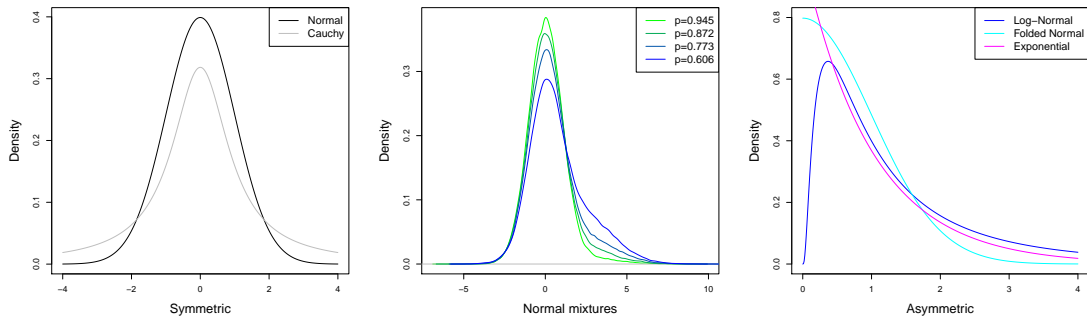
Fig. 1: The left figure shows the symmetric Normal and Cauchy density curves. The middle figure shows the density curves of Normal mixtures of the form pN(0, 1) + (1 - p)N(2, 2) , for 0 < p < 1 . The rightmost figure shows the three ‘highly’ asymmetric densities which, in order of increasing asymmetry, are Log-Normal, Folded Normal and Exponential.
