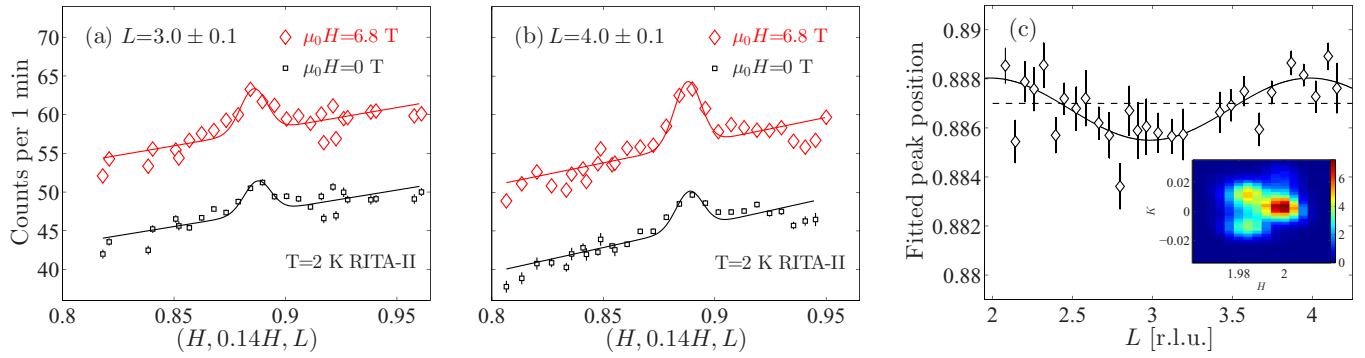
FIG. 2. (Color online) (a, b) Raw data for sample rotation scans through the IC position ( H 0.14H , L ) for L = 3.0 and L = 4.0 in H = 6.8 T (red data points) and zero (black data points) applied field along the c direction, taken at T = 2 K. These data were taken at RITA-II, PSI. For each scan the data of five blades were combined, leading to an uncertainty in L of 0.1 r.l.u. Error bars are smaller than the marker size. The field data are shifted upwards by a constant offset for clarity. The solid curves display fits to Gaussian functions on a sloping background. (c) The fitted peak position H_{IC} for 6.8 T field data as a function of L . The dashed black line shows a fit to a straight line and the solid black line displays a fit to a sine function, which provides a better fit to the data. The color inset shows the intensity of the structural scattering signal around (200) .
