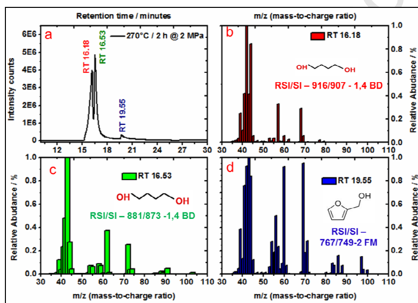
Figure 3 : GC-MS results of the as-synthesised suspension obtained after processing the precursor at 270^\circ\text{C} and 2 MPa for 2 h; (a) the GC spectra; (b), (c) and (d) are the respective MS spectra of the peaks obtained at retention times of 16.18, 16.53 and 19.55 mins, respectively.
