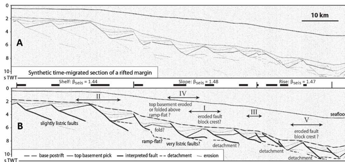
Figure 1. A: Synthetic seismic section across model rifted margin. TWT—two-way traveltime. B: Interpretation showing well-defined fault blocks and synrift wedges bounded by listric faults, which to the right merge into a well-defined detachment system. The crests of several fault blocks appear eroded, suggesting they were near sea level toward the end of rifting. Summing the heaves provides an estimate of the total extension. Most of these interpretations are incorrect: the faults are not so listric, there is no detachment system, the crests of the fault blocks have not been eroded and were not at sea level during late rifting, and the observed fault heaves only show a fraction of the total extension. Roman numerals refer to features shown in Figure 4. \beta_{seis} —seismically derived stretching factor.
