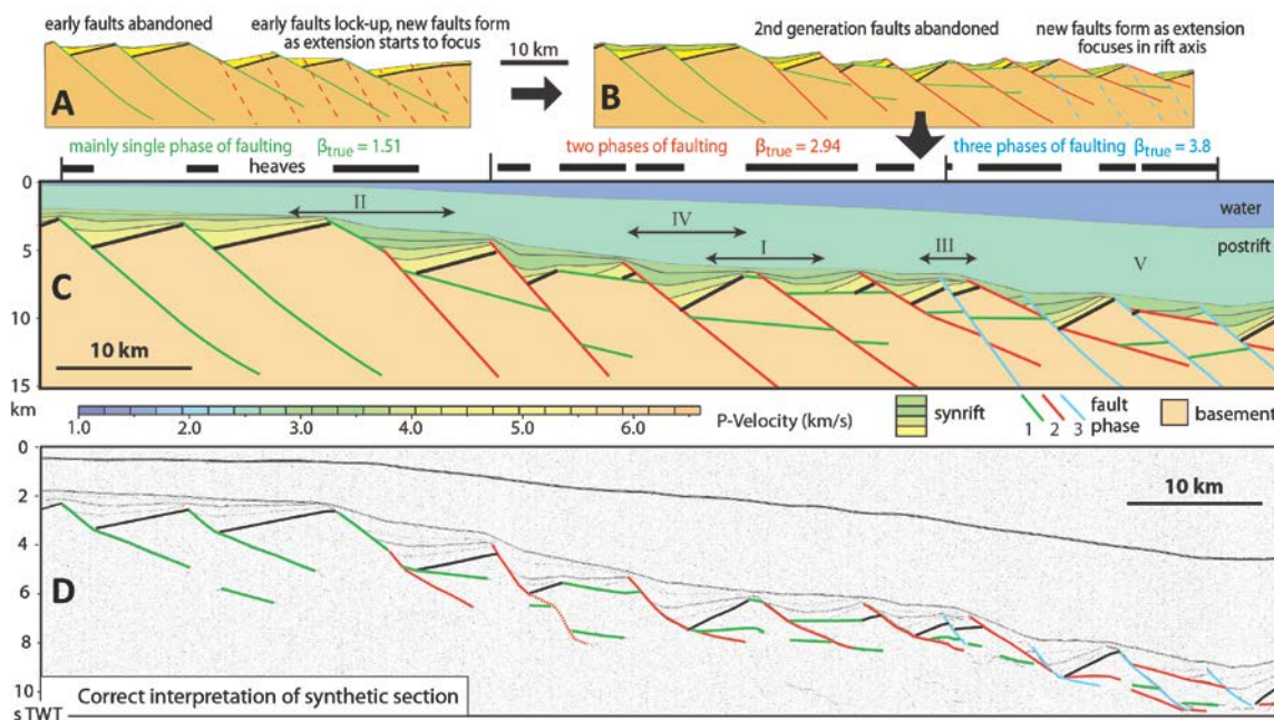
Figure 2. Kinematic model focusing extension in the rift axis via three phases of crosscutting faults, producing complex geometries. A: One side of rift during early extension. Near the rift axis, faults rotate to <40^\circ and become locked; new faults cut across them. \beta_{true} —true stretching factor. B: Extension continues along new faults until these in turn become locked and a third generation of crosscutting faults develops near the axis. C: The final stage, after deposition of a thick postrift sequence (shown unreflective), used to produce the synthetic seismic section (Fig. 1A). Roman numerals refer to features shown in Figure 4. D: The correct interpretation of the synthetic seismic section. Simple structures have been distorted by the overlying velocity structure, the faults are not so listric, there is no detachment system, and the crests of late fault blocks have been shaped by earlier faulting rather than eroded. The total amount of extension is approximately twice that interpreted in Figure 1, with considerably more extension further oceanward. TWT—two-way travelttime.
