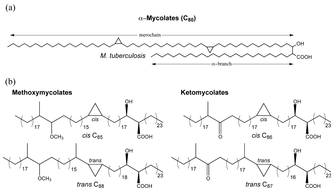
Fig. 1. A. Fundamental structure of a mycolic acid shown using M. tuberculosis \alpha -mycolic acid as an example. B. Structures of other mycolic acid subclasses from M. tuberculosis .
