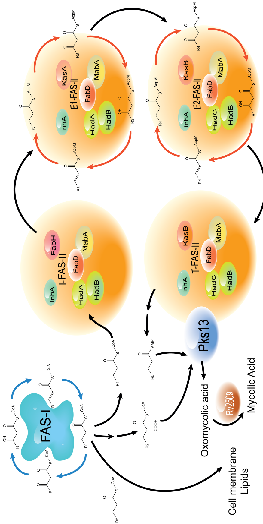
Fig. 2. Schematic illustrating the biosynthesis pathway for mycolic acids in M. tuberculosis in the context of proposed specialised FAS-II complexes. R1; C 16 -C 18 , R2; C 23 -C 26 , R3 represents a range of intermediate length meroacyl chains, R4 represents a range of longer meroacyl chains, R5 is the longest meroacyl chain. I-FAS-II; initiator FAS-II, T-FAS-II; termination FAS-II, and E1-FAS-II and E2-FAS-II represent elongation complexes.
