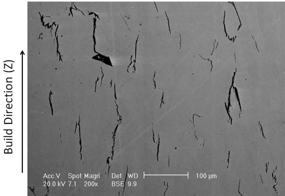
Figure 11: BSE SEM micrograph showing cracked sample with low void percent (150 W, 1500 mm/s, 0.5(a1), 2 mm islands).
