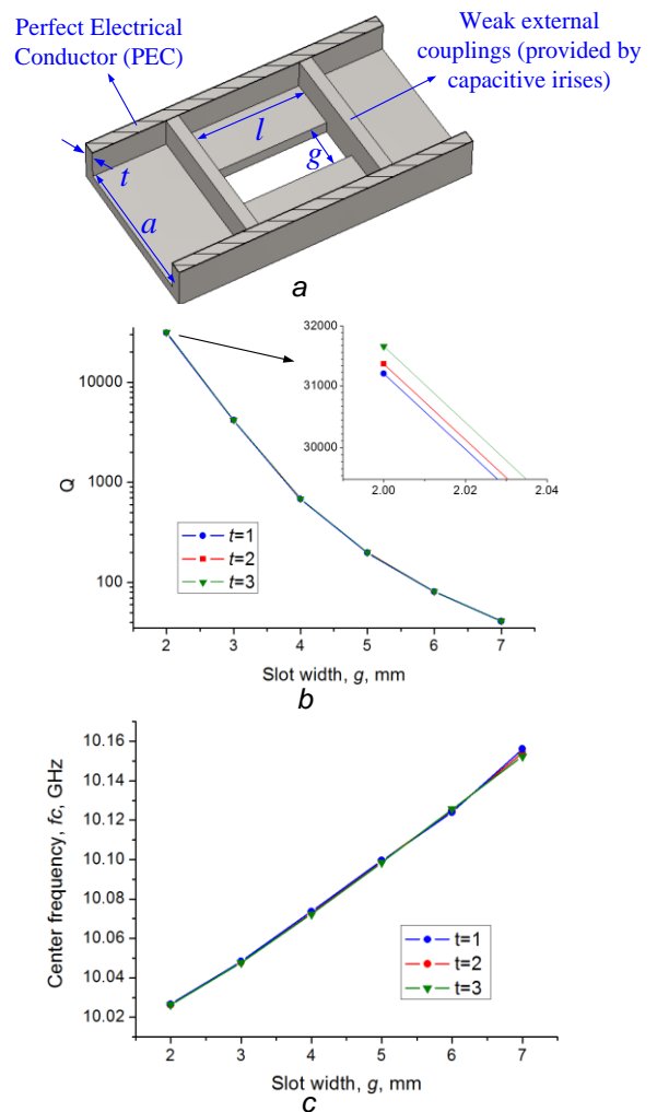
Fig. 2 An X-band TE_{101} cavity resonator with broadside wall slots.
