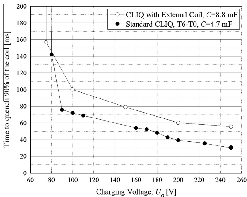
Fig. 14. Calculated time required to quench 90% of the coil versus U_0 , after a standard CLIQ discharge (Configuration T6–T0, C=4.7 mF) or a CLIQ discharge through an external coil ( C=8.8 mF) at I_0=200 A.
