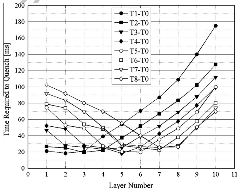
Fig. 10. Calculated time required to quench 90% of each of the ten layers of the solenoid magnet after a CLIQ discharge for various configurations (T1–T0 ··· T8–T0, I_0 = 200 A, U_0 = 75 V, and C = 8.8 mF).
